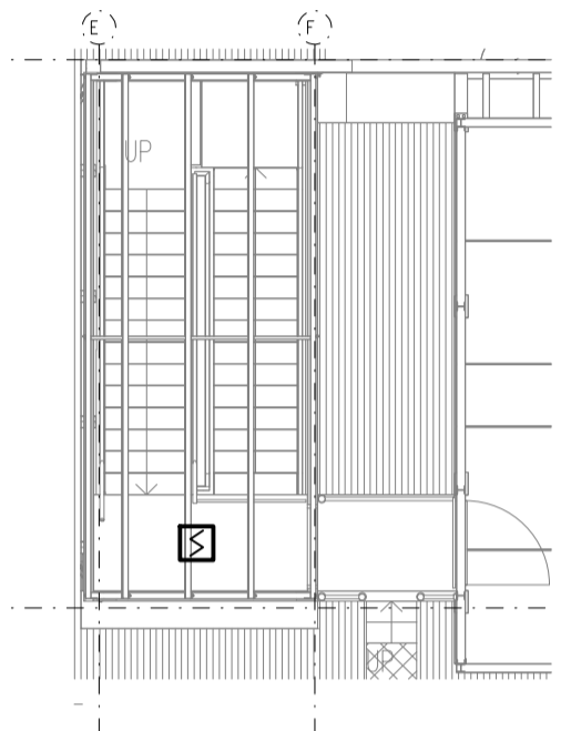
MEZZANINE STAIRS UP TO ROOF LEVEL SCALE 1:100
