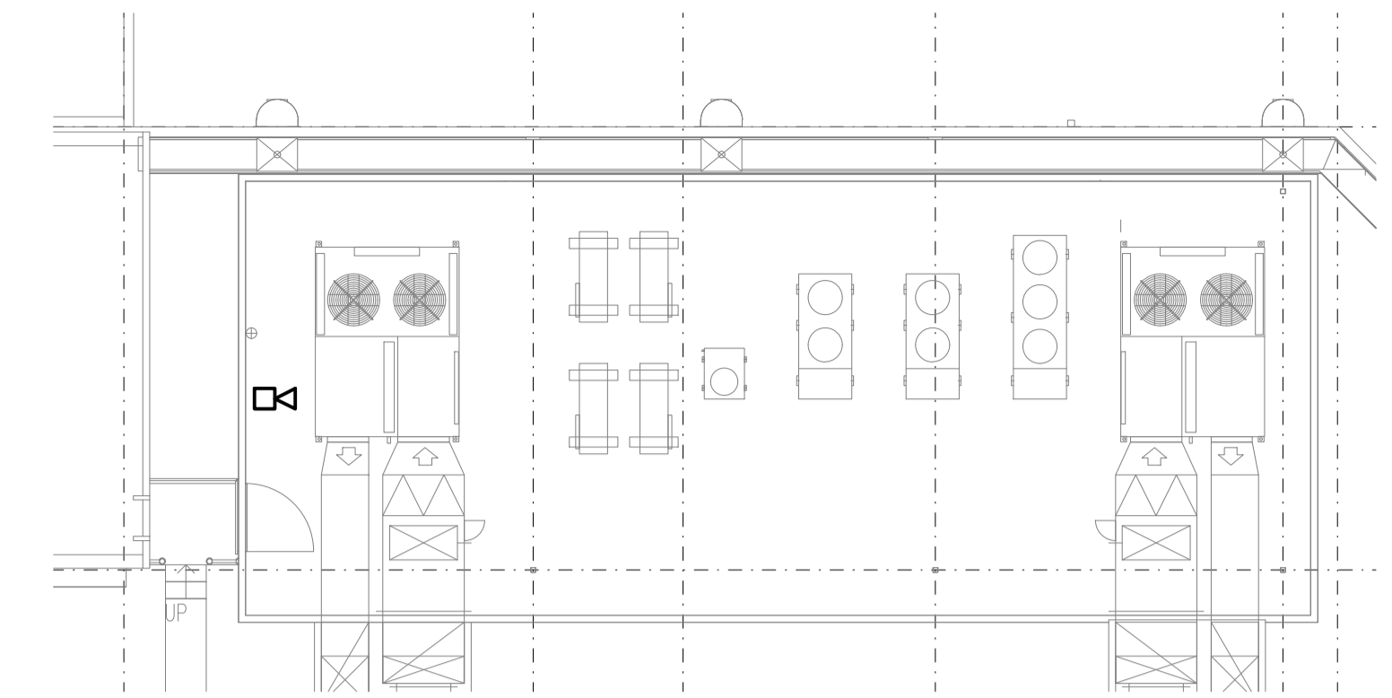
ROOF PLANT DECK SCALE 1:100
